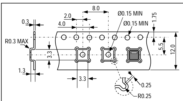
Figure 13 Sketch of packaging tape and sensor orientation.
