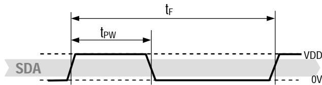
Figure 9 PWM signal. Base frequency runs constantly at approximately 120 Hz, hence t_F is about 8.3ms. The signal is provided on t_{PW} as a ratio of t_F .
