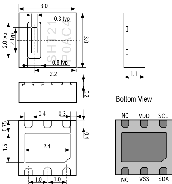
Figure 1: Drawing of SHT21P sensor package, dimensions are given in mm (1mm = 0.039inch), tolerances are \pm 0.1 mm. NC and die pad (center pad) are internally connected to VSS. They may be left floating. VSS = GND, SDA = DATA.
