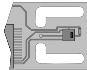
Figure 7 Top view of example of mounted SHT21P with slits milled into PCB to minimize heat transfer.
